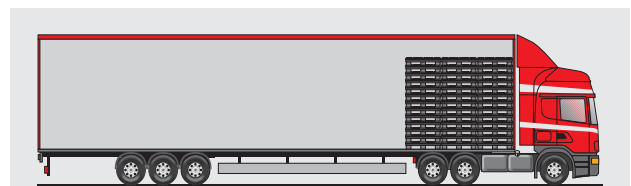
Return shipping (mega trailer): 78 empty ROBUPAC systems (1200 x 800) on approx. 3 loading meters
